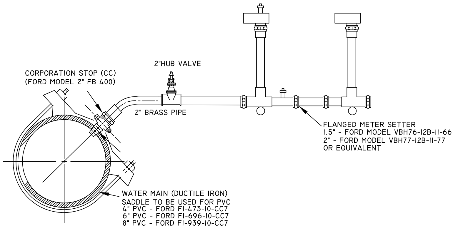
LONG SIDE METER CONNECT
