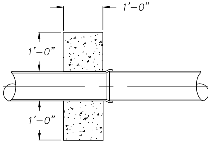
TYPICAL SECTION CONCRETE ANCHOR
