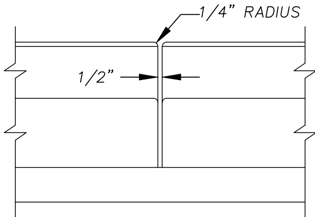
TYPICAL EXPANSION JOINT
