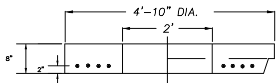
SECTION, 4' COVER SLAB
