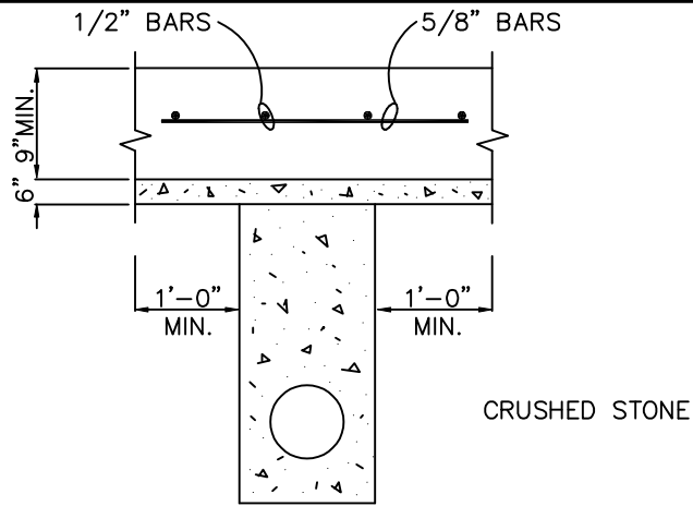
CONCRETE PAVEMENT
