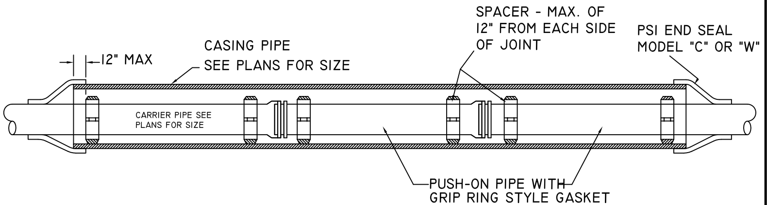
TYPICAL CASING SPACER INSTALLATION
