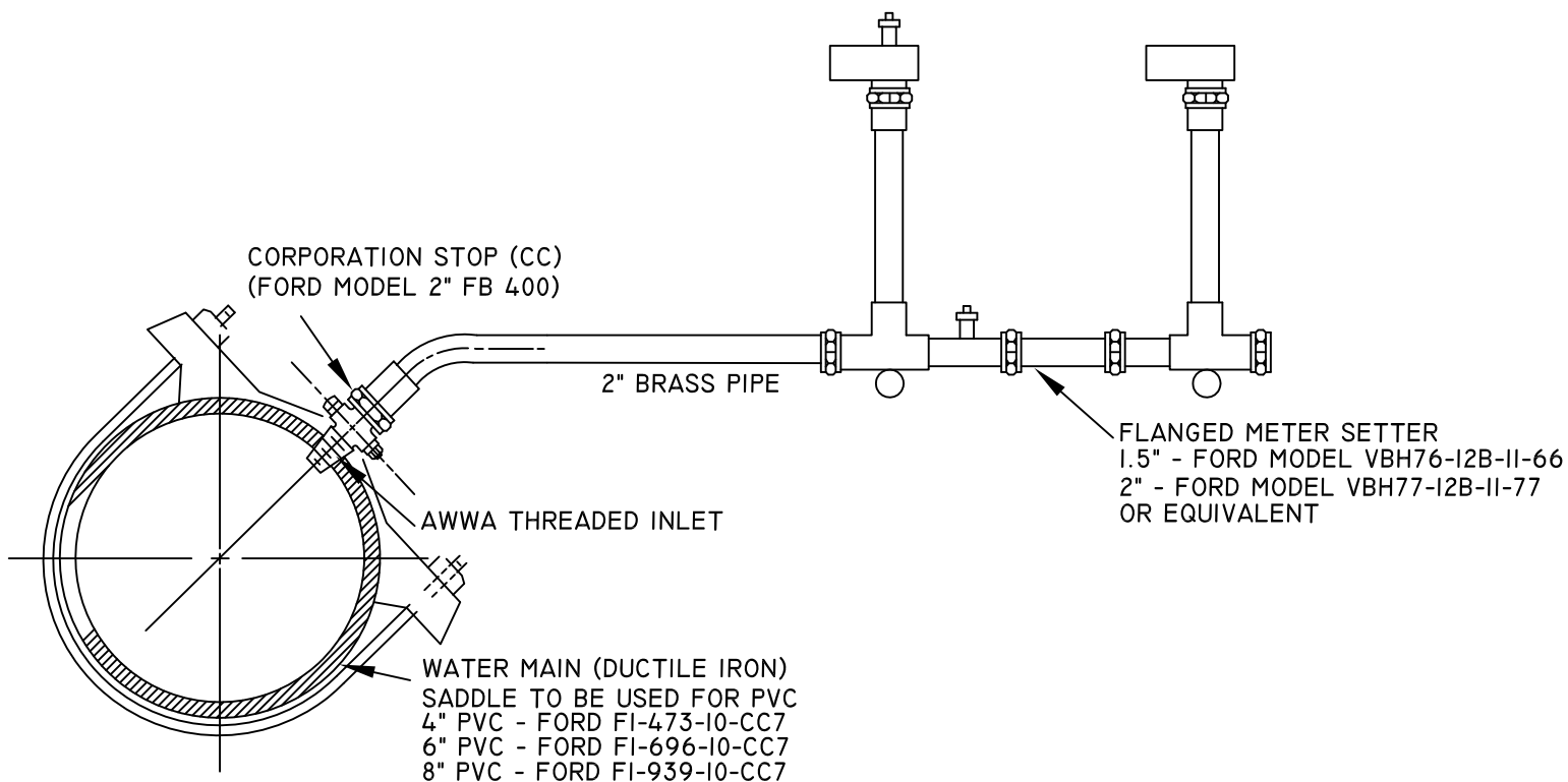
SHORT SIDE METER CONNECT
