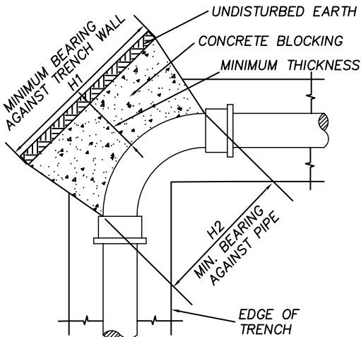
HORIZONTAL BENDS
