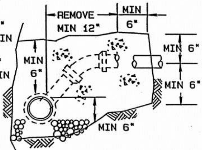
FIELD ADAPTED SERVICE CONNECTION
