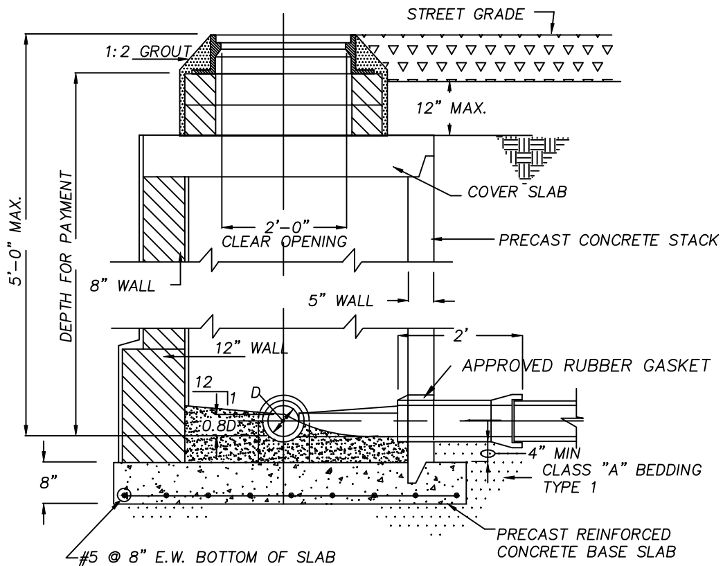
SECTION, USING PRECAST CONCRETE STACK
