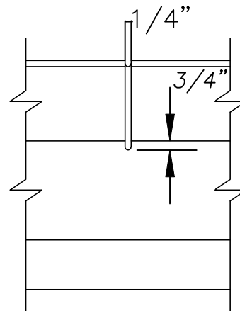
TYPICAL CONTRACTION JOINT
